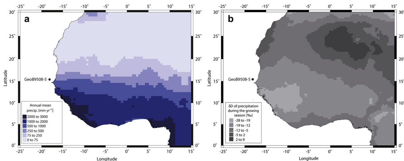
Fig. 2. (a) Mean annual rainfall over tropical northwest Africa. Graphic is based on a compilation of rainfall data from the period 1950–1999 available on the Willmott, Matsuura and Collaborators Global Resources Pages ( http://climate.geog.udel.edu/~climate/ ), Center for Climatic Research at University of Delaware. (b) Stable hydrogen isotopic composition ( \delta D ) of precipitation over tropical northwest Africa during the growing season. Graphic is based on data from www.waterisotopes.org (Bowen and Revenaugh, 2003; Bowen, 2009).
