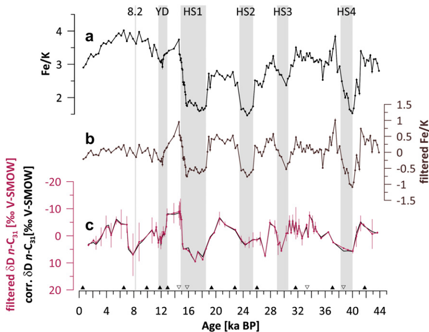
Fig. 4. Temporal variability of (a) the Fe/K record from the same core (Mulitza et al., 2008), (b) the Fe/K record and (c) the \delta\text{D} record both after high-pass filtering (Rybicki and Press, 1995) with a cut-off frequency of 1/(10,000 \text{ yr}) to show variability other than linked to insolation. Gray bars indicate periods of Heinrich stadials (HS, after Sarnthein et al. (2001)), the Younger Dryas interval (YD) and the “8.2 ka” event. Filled triangles indicate age points derived by radiocarbon dating, open triangles indicate age points derived by correlation with the benthic \delta^{18}\text{O} record of core MD95-2042 (Mulitza et al., 2008). Error bars ( 1\sigma ) are given for multiple-measurements only.
