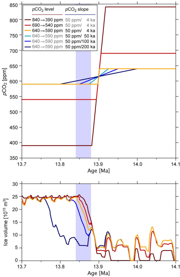
Fig. 7. p\text{CO}_2 sensitivity experiments – level of initial and final p\text{CO}_2 (yellow to red colors) and rate of p\text{CO}_2 decrease (blue colors). Colors in upper panel show p\text{CO}_2 forcing and correspond to ice-volume transition in lower panel. Blue box indicates approximate Antarctic glaciation as retrieved from sedimentary records. Glaciation is independent from initial and final p\text{CO}_2 levels (red to orange). On the contrary, the rate of the p\text{CO}_2 drawdown is important. Extremely slow drop in p\text{CO}_2 (dark blue) results in delayed ice-sheet extension, relatively slow decrease (light blue) causes appropriate timing with glaciation. A p\text{CO}_2 drop of 50 ppm/50 ka or faster (for example 50 ppm/4 ka in orange) gives the same ice-sheet transition as 50 ppm/50 ka.
