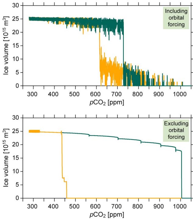
Fig. 3. Hysteresis experiment. Starting from no-ice conditions and high p\text{CO}_2 (orange) or starting from full ice sheet and low p\text{CO}_2 (green). Upper panel shows hysteresis including orbital forcing, lower panel without orbital variations. Rate of p\text{CO}_2 change is 280 ppm/5 Ma.
