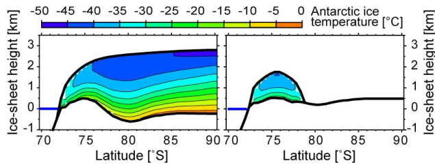
Fig. 5. Cross-section of large (left) and small (right) Antarctic ice sheets. Color scale corresponds to annual mean ice temperatures.
