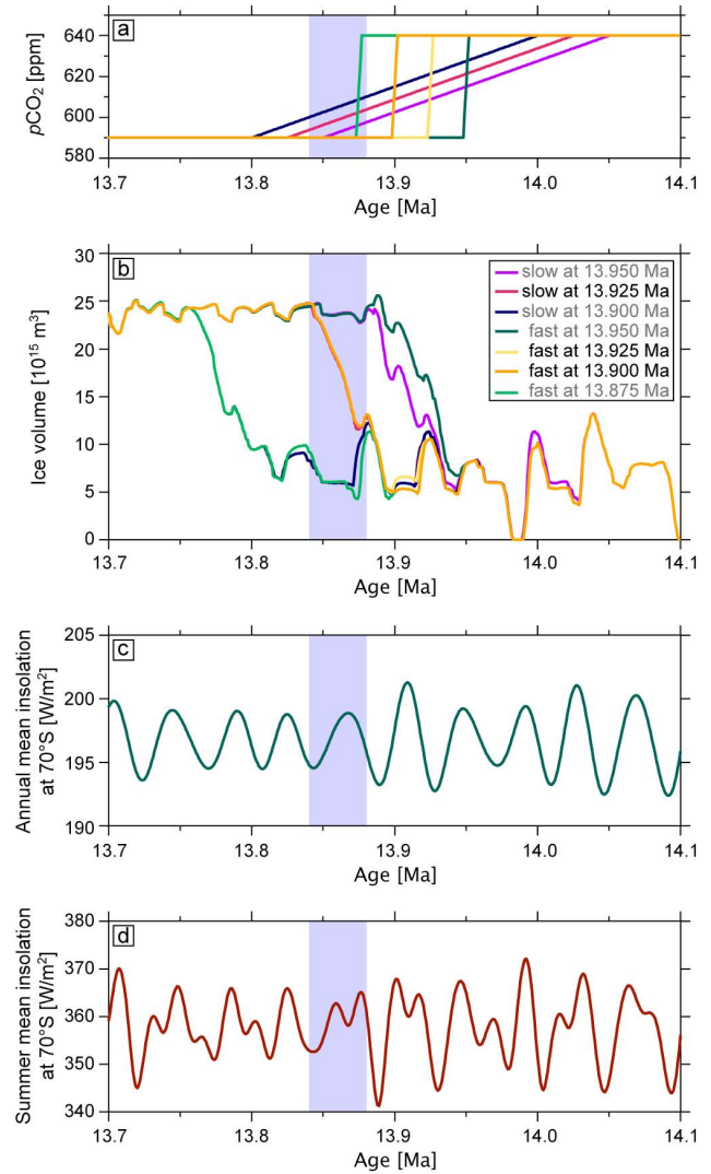
Fig. 8. p\text{CO}_2 sensitivity experiment – timing of p\text{CO}_2 decrease. Colors in (a) show p\text{CO}_2 forcing and correspond to ice-volume transition in (b). Blue box indicates approximate Antarctic glaciation as found in sedimentary records. Green/orange curves result from fast p\text{CO}_2 transition (50 ppm/4 ka); purple/blue ones from a slow drop (50 ppm/200 ka). Black (gray) text in legend indicates best (not) fitting solutions (see Discussion section). Orange and dark blue curves correspond to their counterparts in Fig. 7. (c) Annual mean insolation at 70° S. (d) Summer mean insolation at 70° S.
