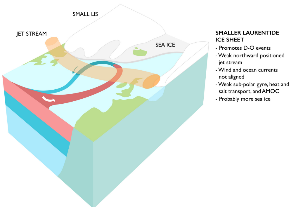
Figure 5. Schematic of a potentially D–O-type oscillating state.
