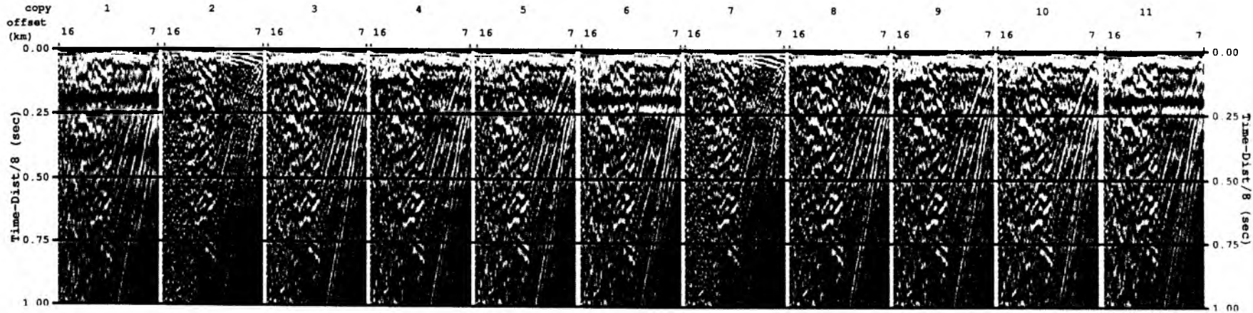
Figure 5.2.2.4: Deconvolution test with autocorrelation functions from record section obh 89 for offset range 7-16 km, Profile 06.
