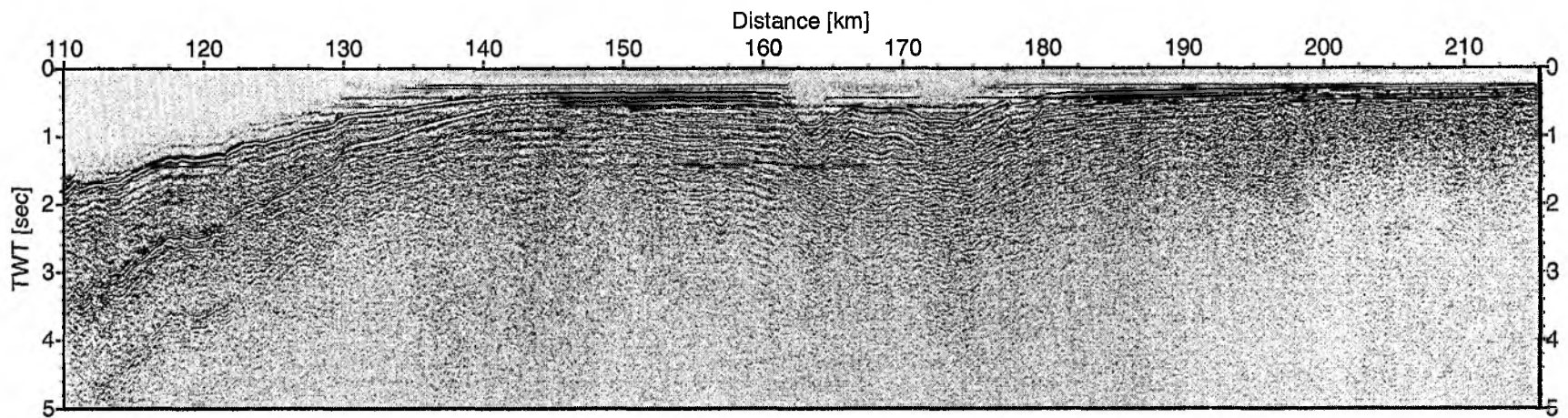
W SO181 Streamer Profile 08 water-migration E
