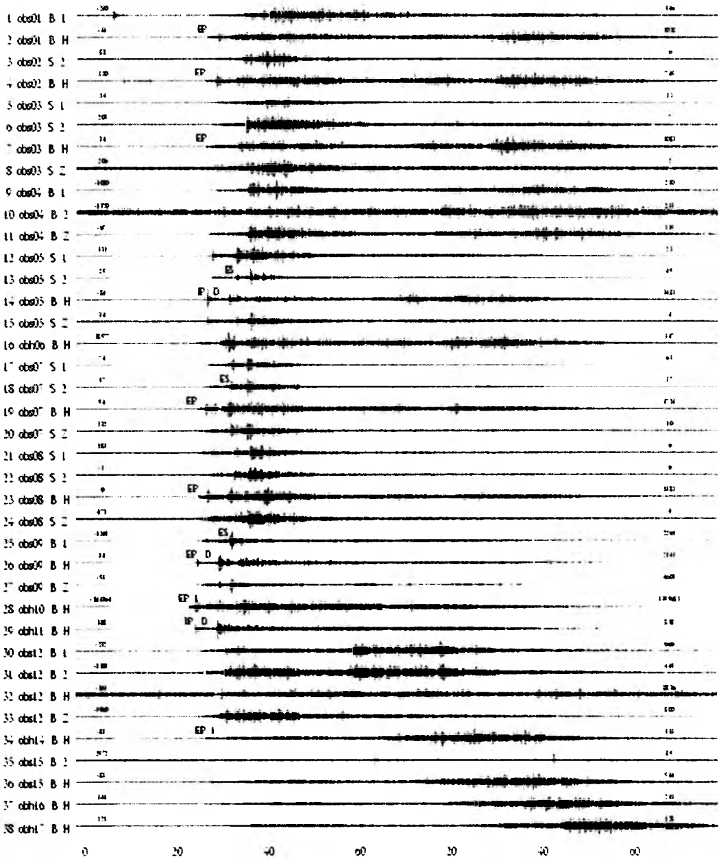
Figure 6.6.1.42: Earthquake from 14 Dec 2004, 18:11 UTC accompanied by T-waves. The event was located 23 km east of OBH 10 at 42.777° S, 75.997° W.
