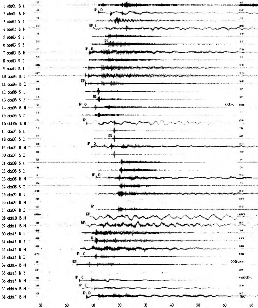
Figure 6.6.1.41: Another deep focus event from 06 Jan 2005, 21:48 UTC located outside the network 33 km south of OBH 14. This earthquake may belong to the swarm detected in the area south of OBH 14.
