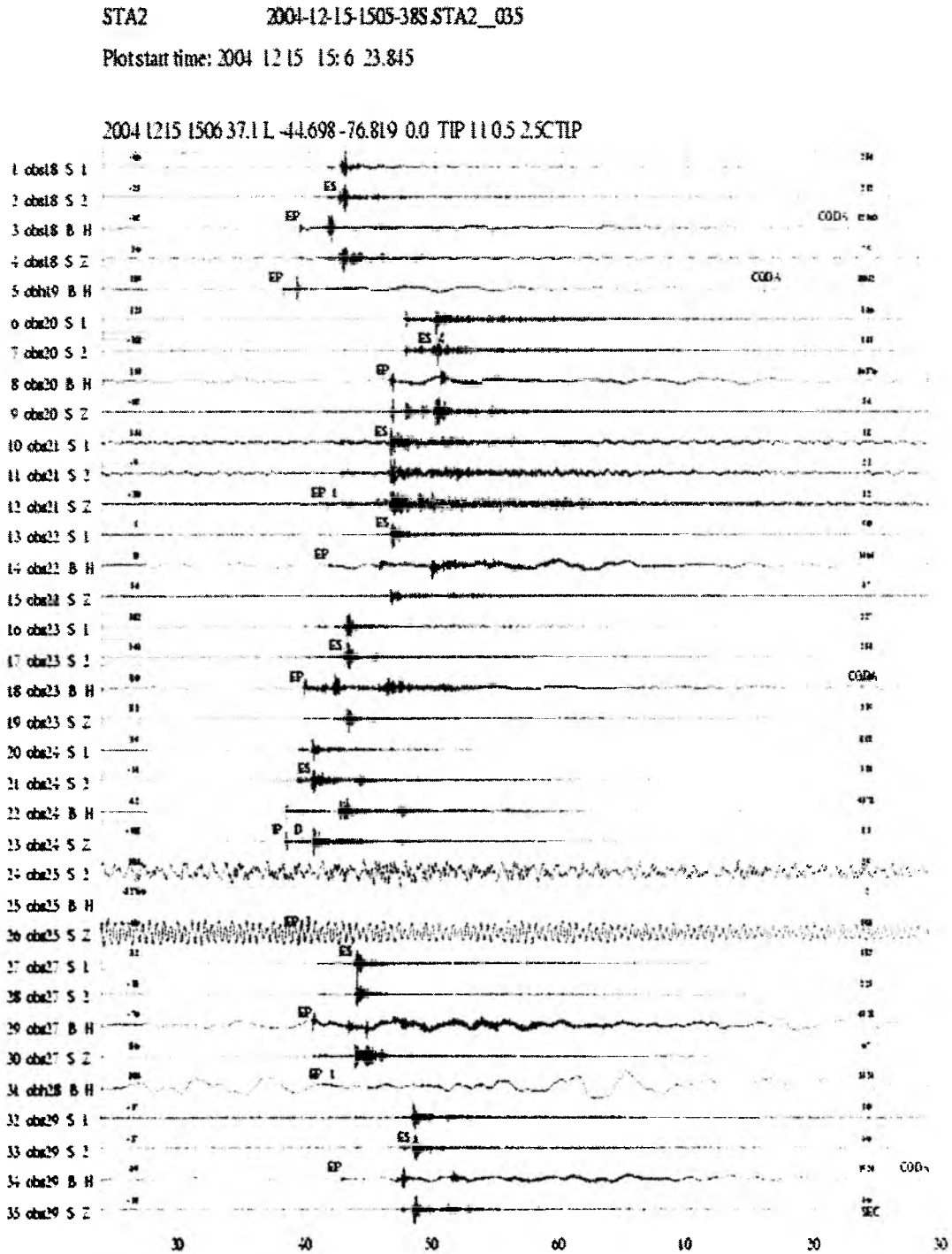
Figure 6.6.148: Inner network earthquake from 15 Dec 2004, 15:06 UTC located at 44.698°S, 76.819°W at the ocean bottom. See the previous subsection for the reliability of the depths of these shallow earthquakes.
