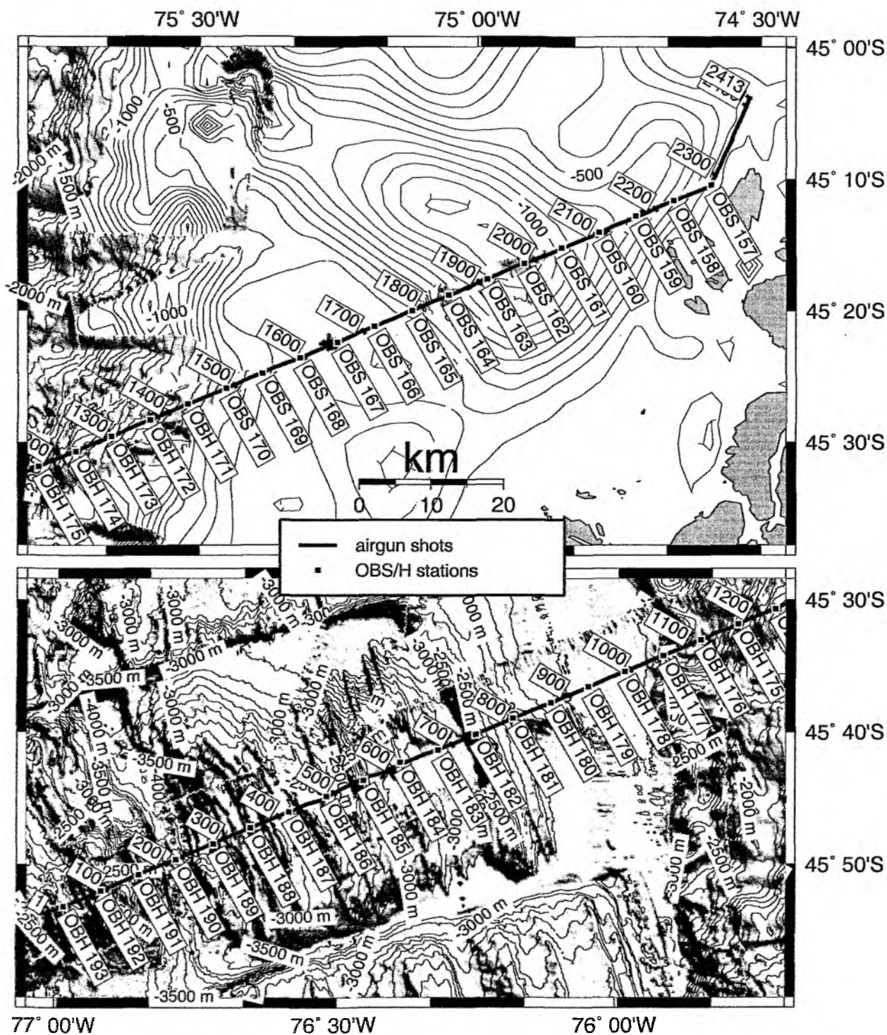
Figure 6.6.5.1: Basemap of P08; transect of ocean bottom seismometer and hydrophone stations and line of airgun shots. Bathymetry contours every 100m.
