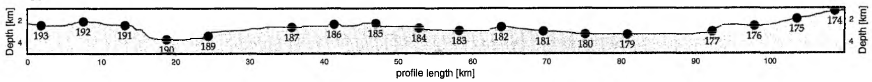
W SO181 Streamer Profile 08 water-migration E
