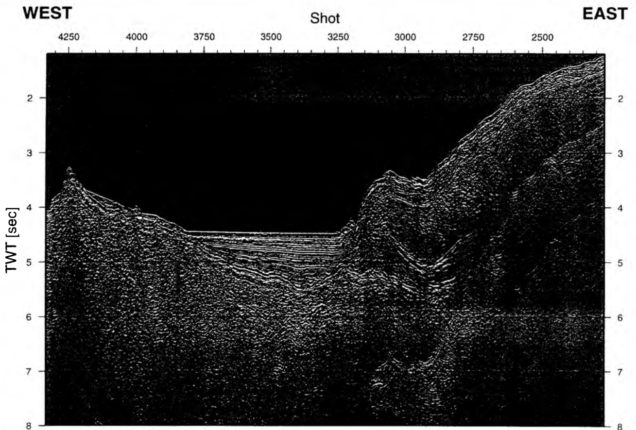
Figure 2.1.3: Line 743 of Lamont-Doherty Earth Observatory's Conrad cruise in 1988. This finite-difference migrated section is located on TIPTEQ corridor 4, imaging the structures from last spreading ridge before the trench to the sediments of the shelf.
