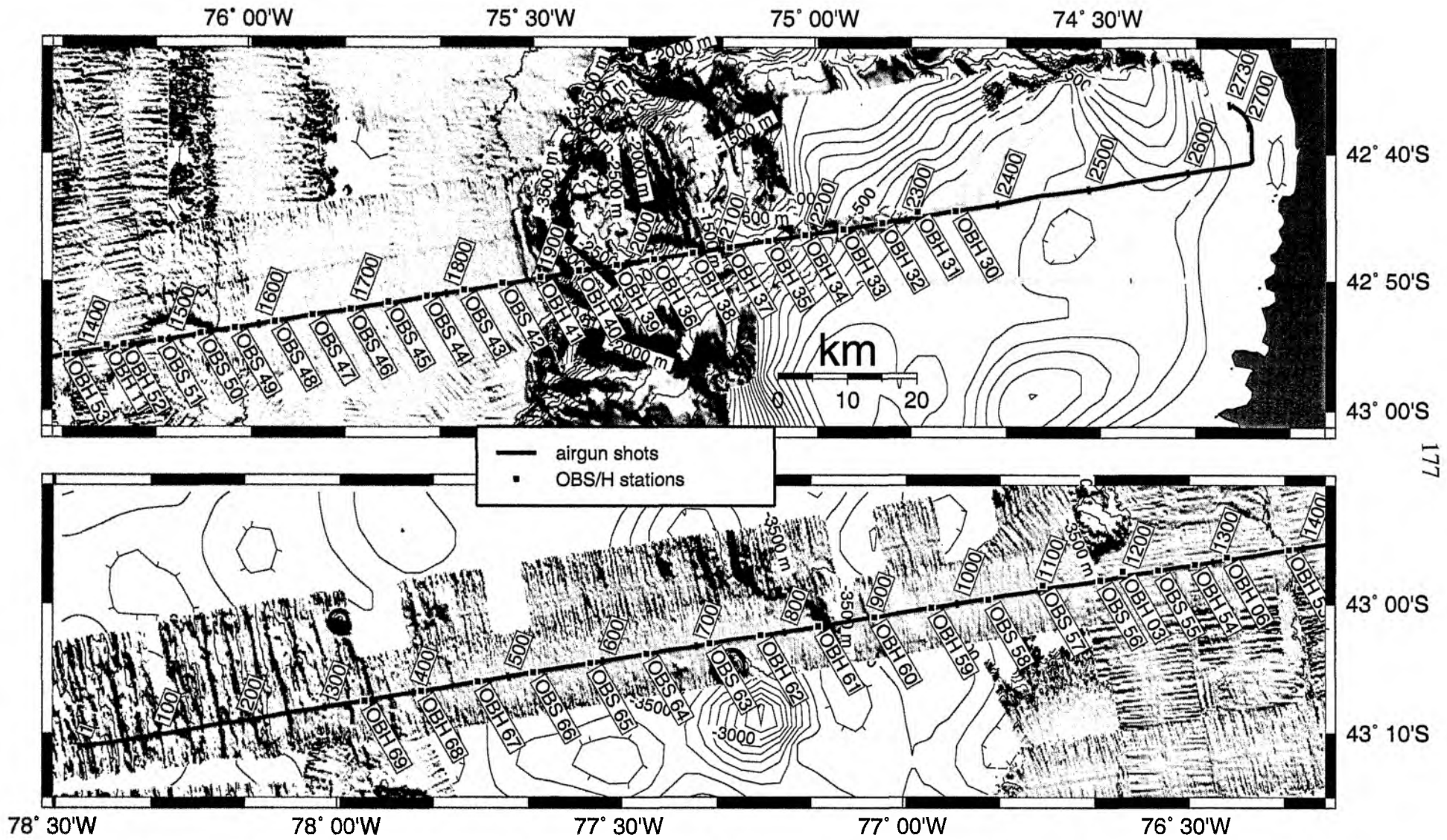
Figure 6.6.3.1: Basemap of P05; transect of ocean bottom seismometer and hydrophone stations and line of airgun shots. Bathymetry contours every 100m.
