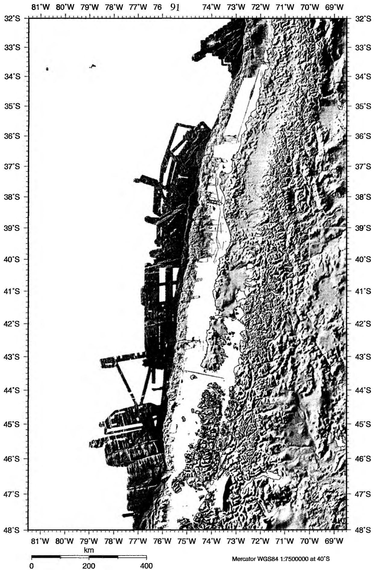
Figure 6.1.3: SO181 bathymetry merged with data from other cruises
