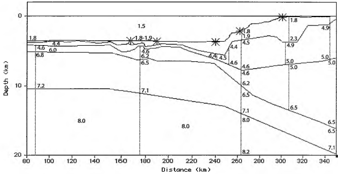
Figure 6.6.3.52: Preliminary model of profile P05 stretching E-W. Stars mark the stations used to create the model.
