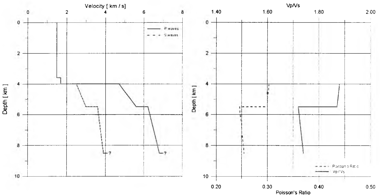
Figure 6.6.1.33: Velocity-depth model for OBH 11 on profile P02.
