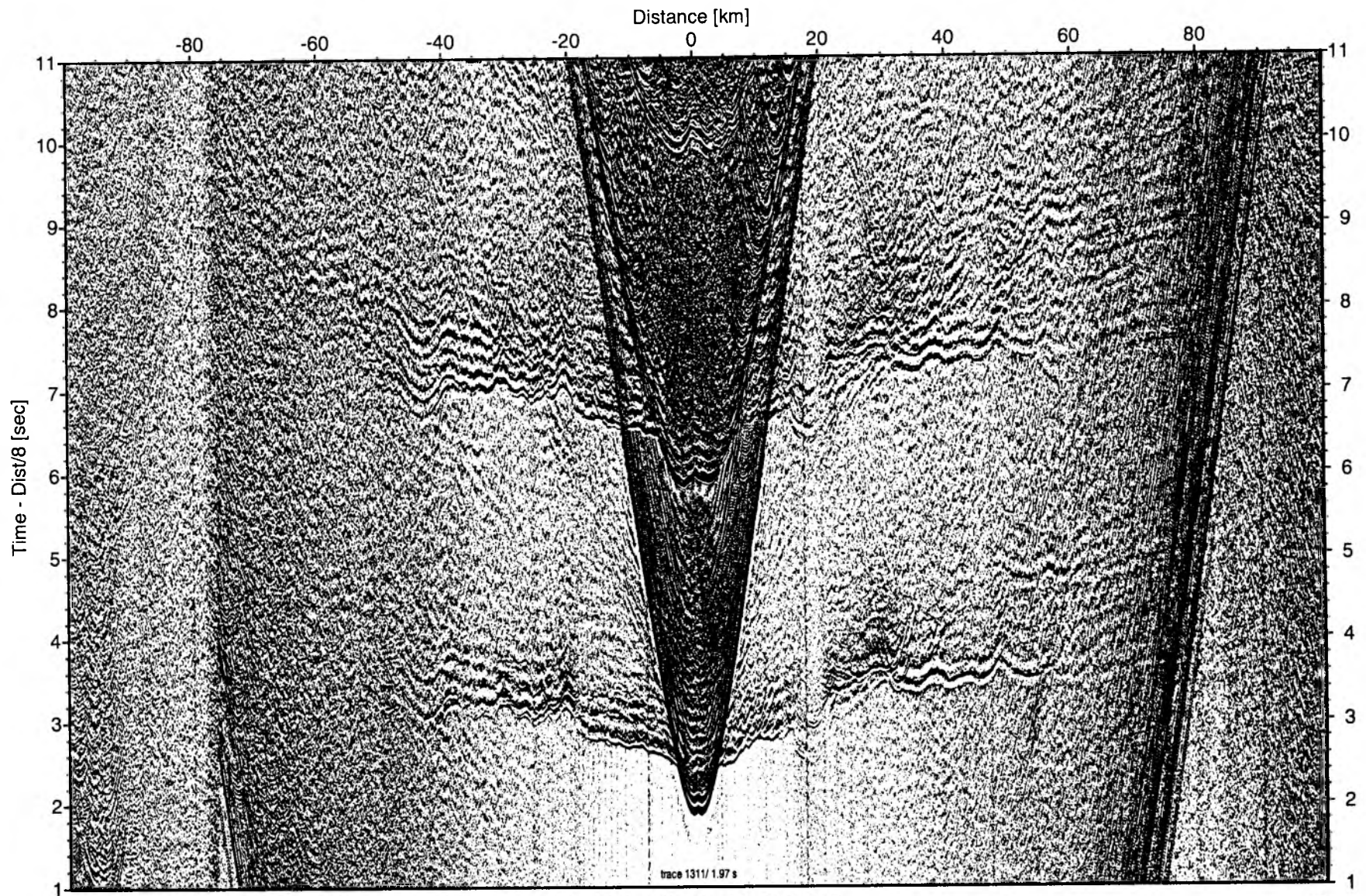
SO181 Profile 06 obh 105 HTI
