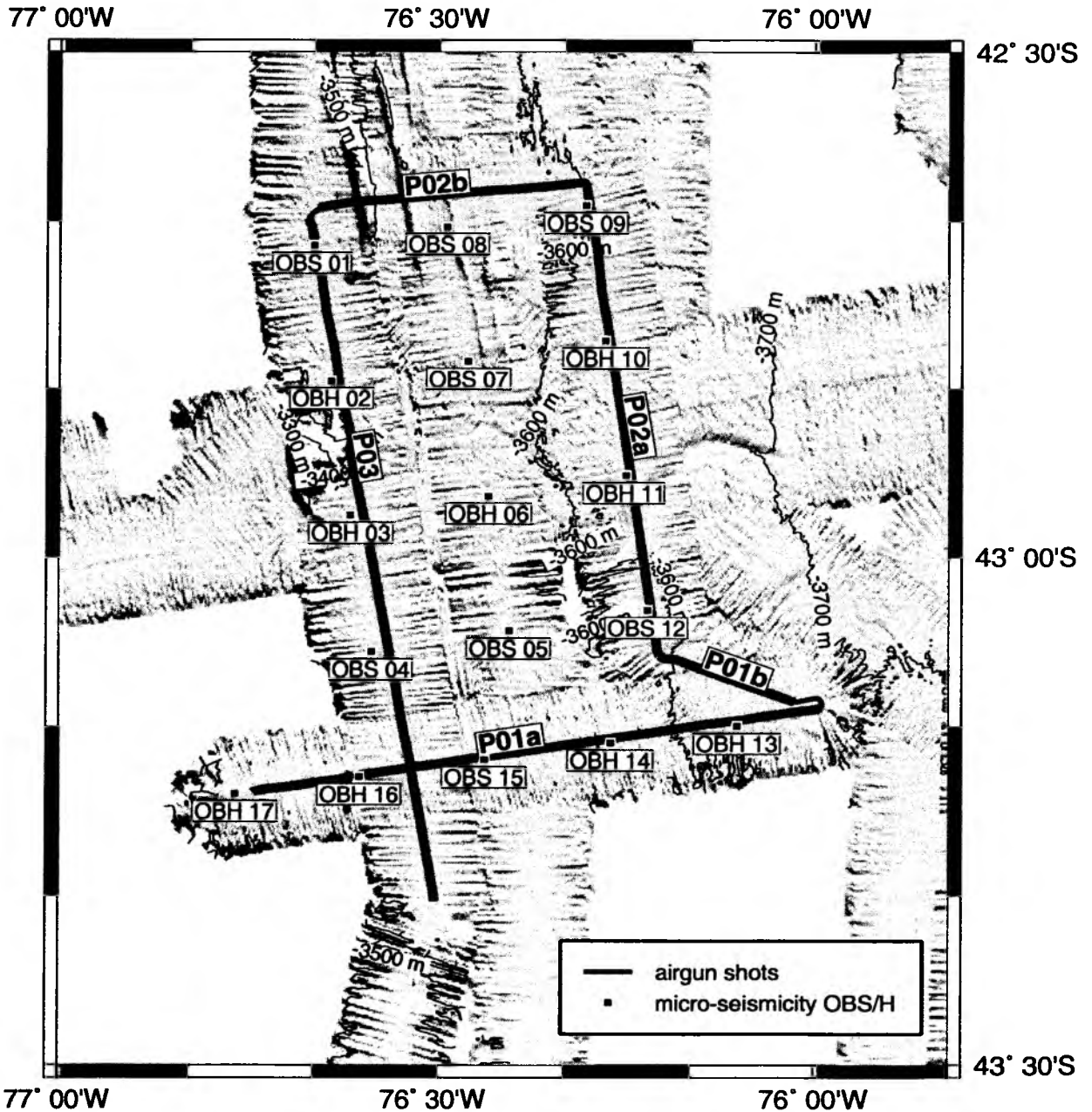
Figure 6.6.1.1: Basemap of short-term array (STA) 1 of ocean bottom seismometer and hydrophone array to study outer rise micro-seismicity. Also shown are airgun profiles. Thicker grey lines mark streamer profiles. Bathymetry contours every 100m.
