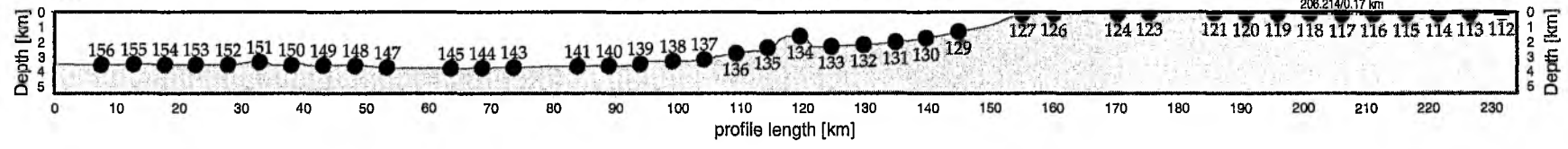
W SO181 Profile 07 obs 117 OAS E
