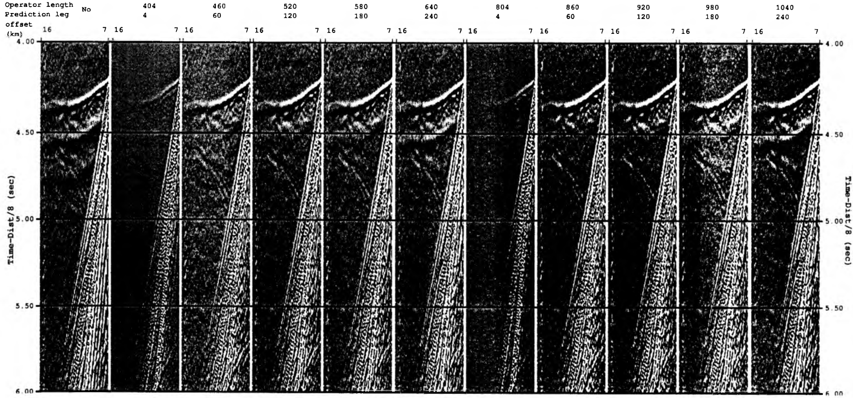
Figure 5.2.2.4: Deconvolution test with autocorrelation functions from record section obh 89 for offset range 7-16 km, Profile 06.
