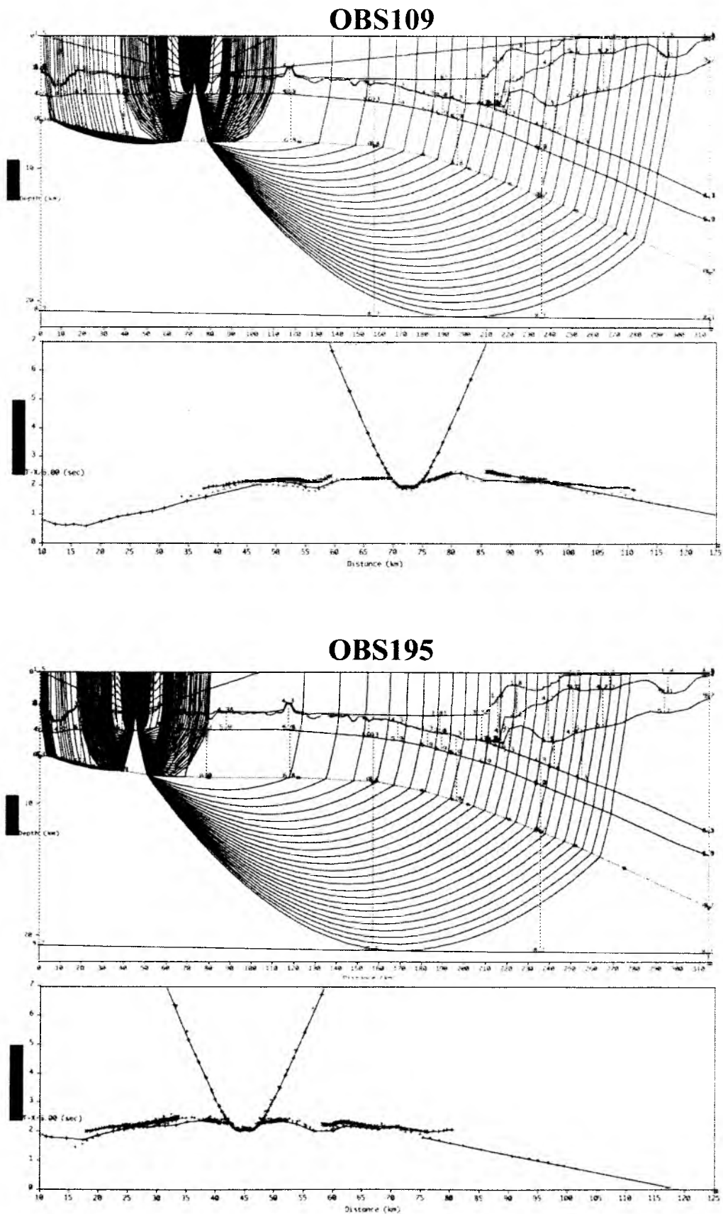
Fig 6.6.67 : raypaths and traveltimes picks of OBS109 and OBS195
