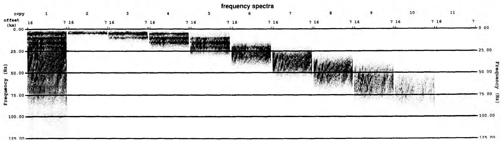
Figure 5.2.2.3: Frequency analysis from record section obh 89 for offset range 7-16 km, Profile 06.
