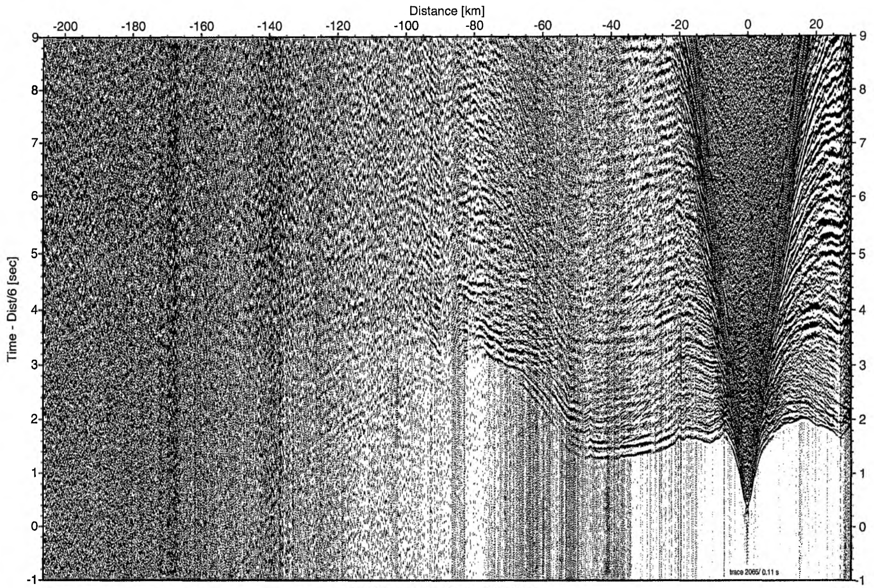
W SO181 Profile 07 obs 117 OAS E
