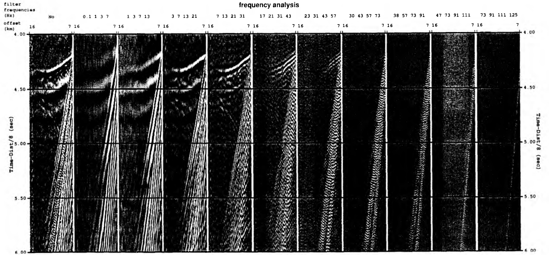
Figure 5.2.2.3: Frequency analysis from record section obh 89 for offset range 7-16 km, Profile 06.
