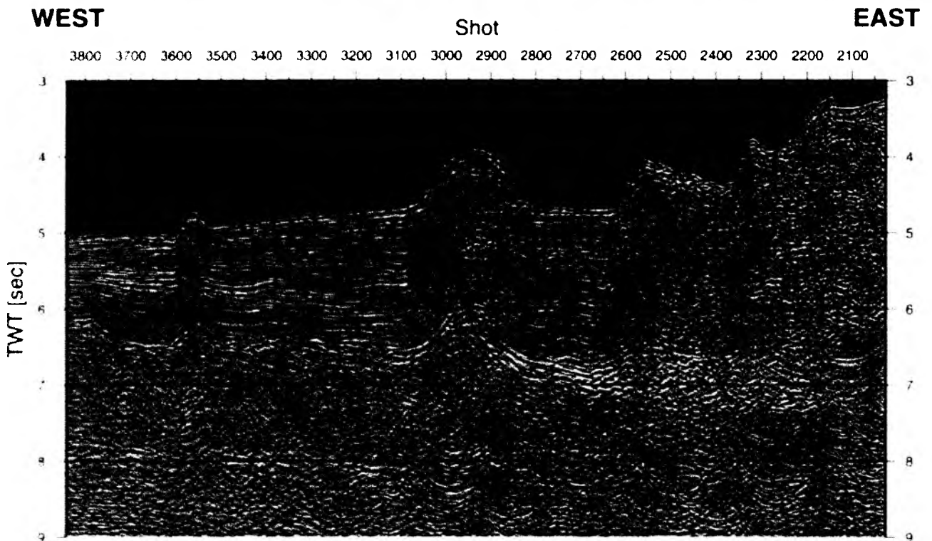
Figure 2.1.4: Line 769 of Lamont-Doherty Earth Observatory's Conrad cruise in 1988. This finite-difference migrated section is located on TIPTEQ corridor 5, imaging the deformation front and the accretionary wedge south of the Chile Triple Junction.
