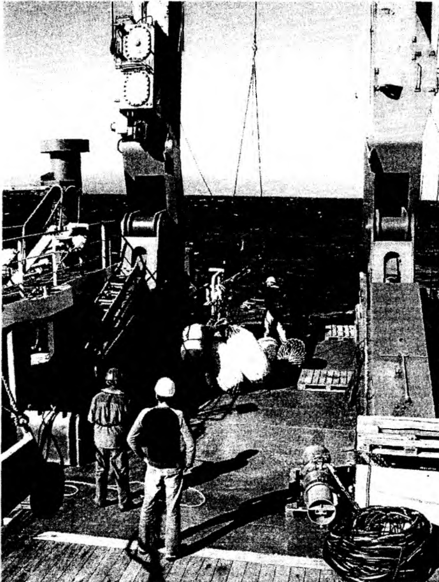
Figure 5.3.10: Starboard side G-gun carrier during recovery The gun frame is lifted by the hoisting rope with its extension operated by the port side mooring winch through the centre block in the A-frame. Starboard towing wire can be seen towards the top left where it passes through a roll on the outside part of the A-frame
